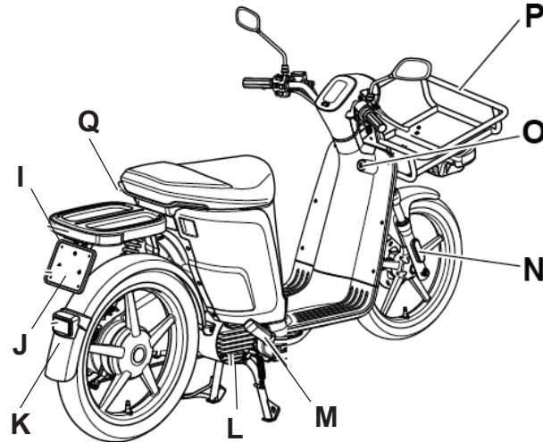
eSPROK1 2 Seats right side
